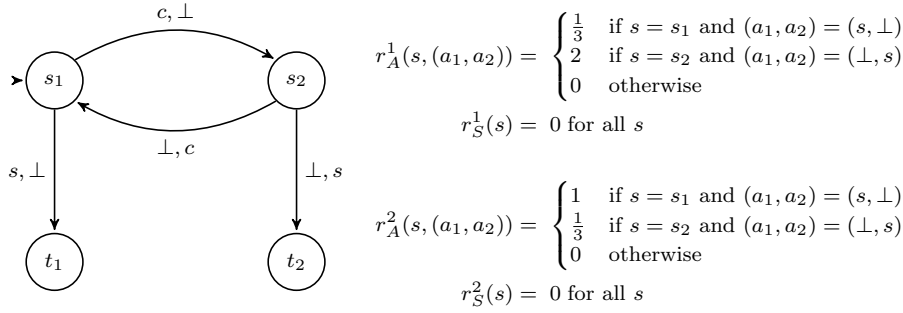
Fig. 14: Counterexample for nonzero-sum expected reachability properties.
