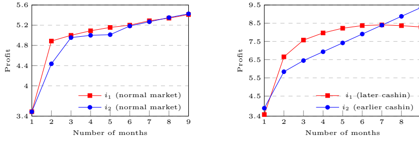
Fig. 8: Futures market: normal profiles (left) and mixed profiles (right) ( p_{\text{bar}}=0.1 ).
