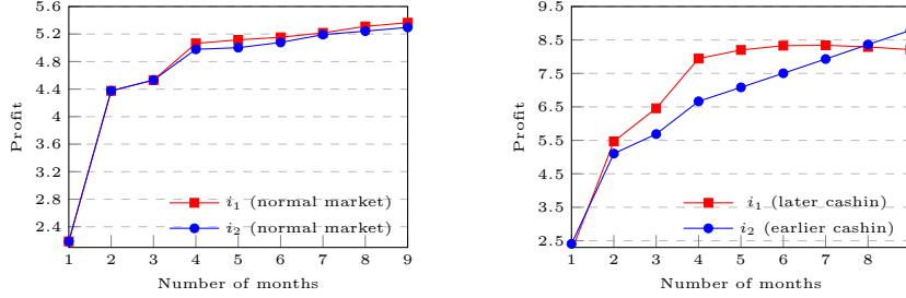
Fig. 9: Futures market: normal profiles (left) and mixed profiles (right) ( p_{\text{bar}}=0.5 ).
