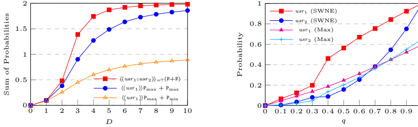
Fig. 11: Aloha: \langle\langle usr_1:\{usr_2, usr_3\}\rangle\rangle_{\max=?}(\mathbb{P}[F(s_1 \wedge t \leq D)] + \mathbb{P}[F(s_2 \wedge s_3 \wedge t \leq D)])
