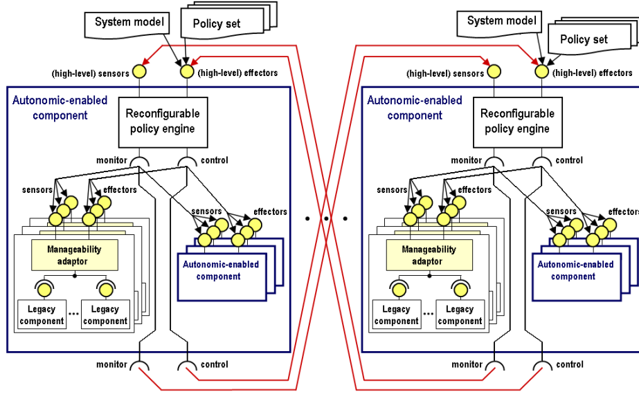
Fig. 2. System-of-systems architecture
