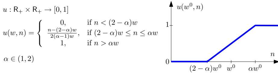
Fig. 3. Sample function u for Example 1 (the graph shows u for a fixed value w^0 of its first argument)
