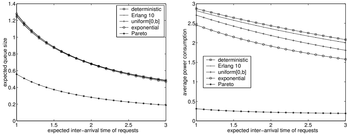
Figure 2: Performance and power results as the expected inter-arrival time varies
